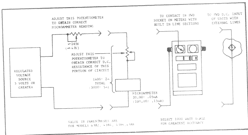
Figure 4.1 Calibration Diagram
